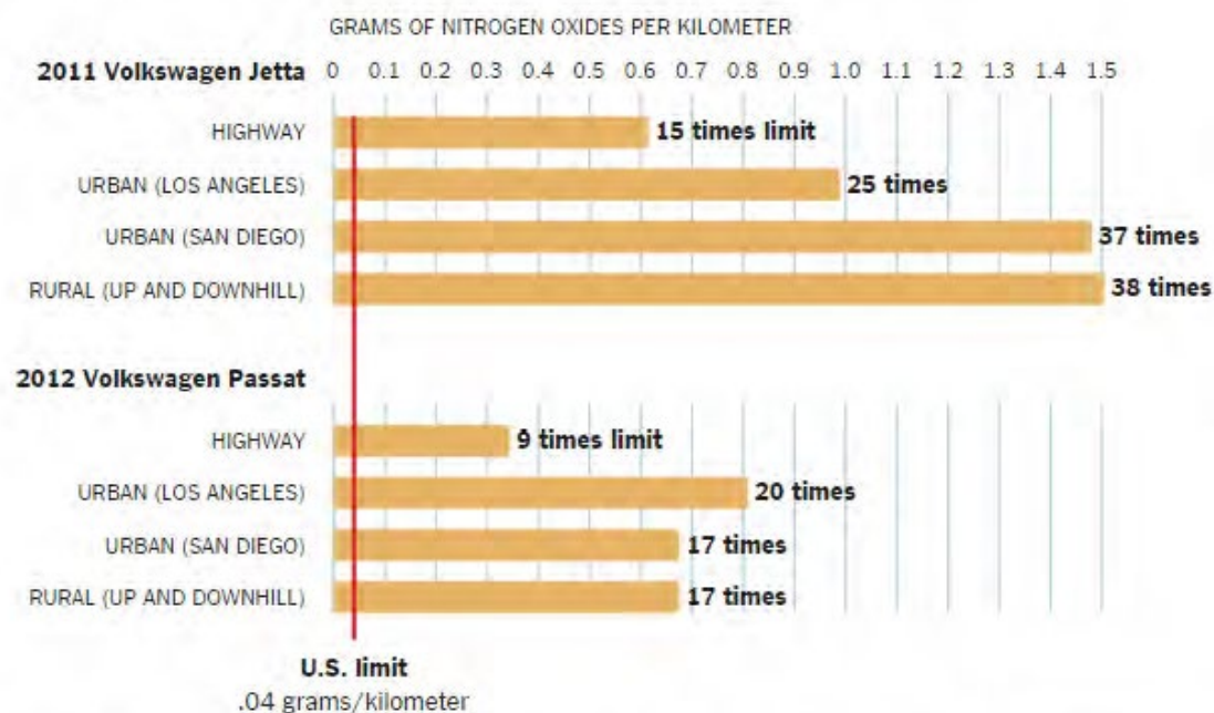
10 Average emissions of nitrogen oxides in on-road testing
