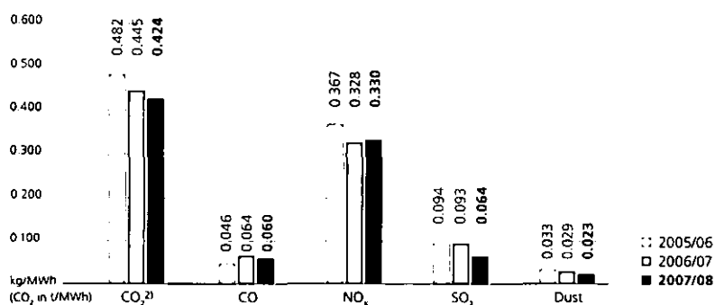
Specific emissions from EVN thermal power stations and district heating plants 1)
